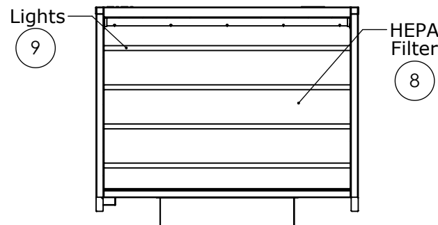
SECTION T-T
