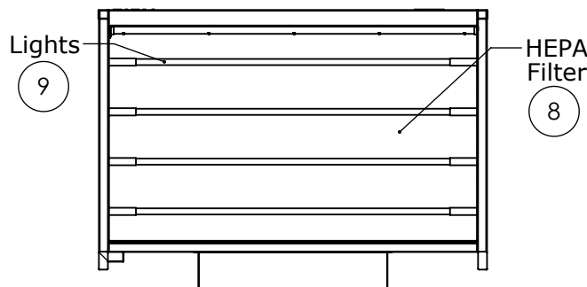
SECTION T-T
